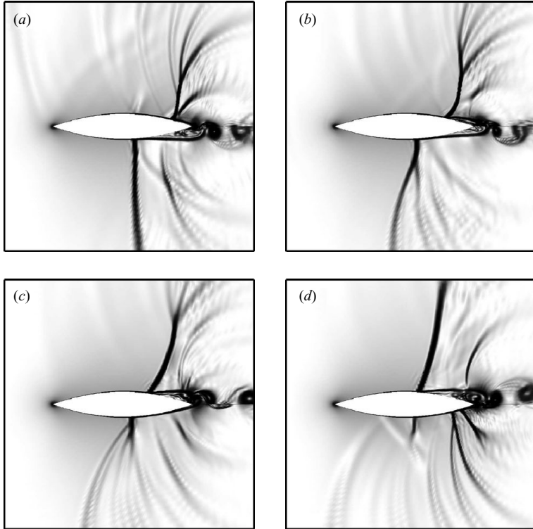
FIGURE 7. Numerical schlieren-like visualization by contours of \|\nabla \bar{\rho}\| in the mid-span ( x, z ) plane during half-period with the same time increment from (a) to (d).
